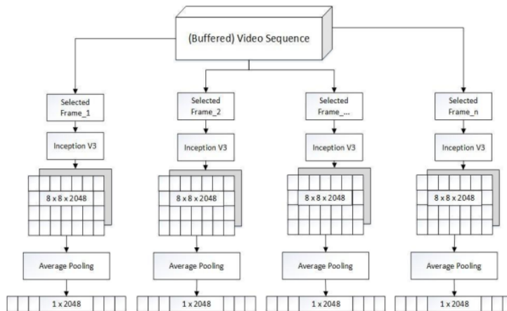
Fig. 3. Inception-v3 feature extraction framework.
