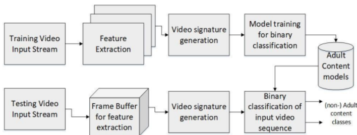
Fig. 2. Proposed architecture for the adult content classification.
