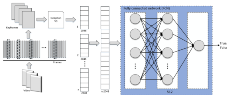
Fig. 4. Fully connected layer model for binary classification.
