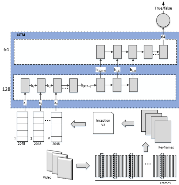
Fig. 5. LSTM layer for binary classification.
